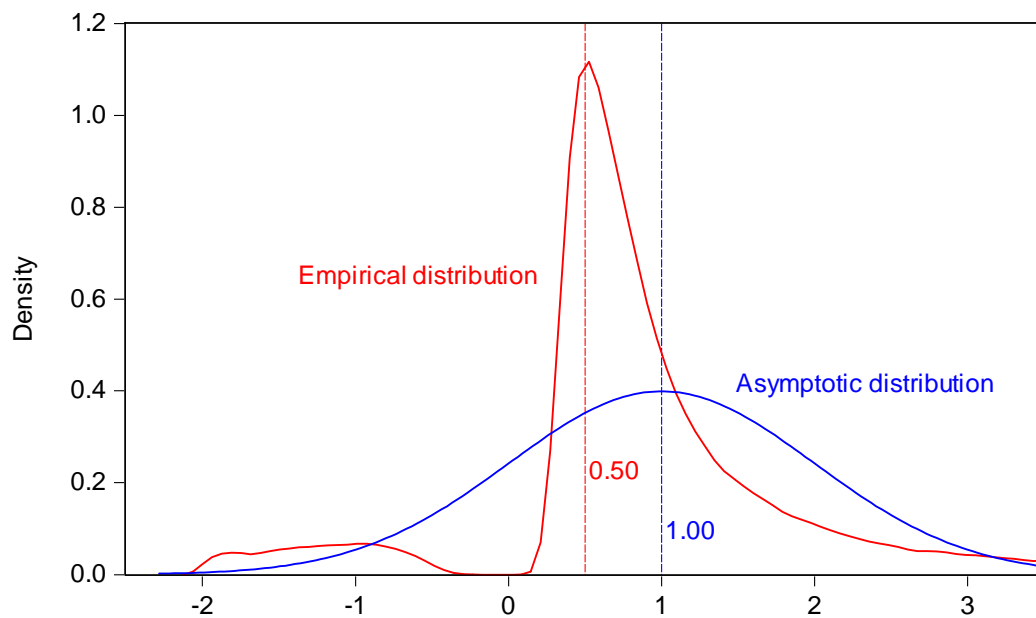
Figure A2. Empirical and asymptotic distributions of “theta” ( \hat{\theta} ), example 2
